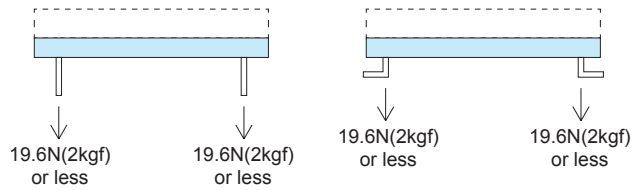
Fig.6.4 Strength of Input/Output Pin Terminals
