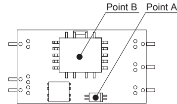
Fig.8.11 Temperature Measuring Points in the case of Forced Air Cooling
