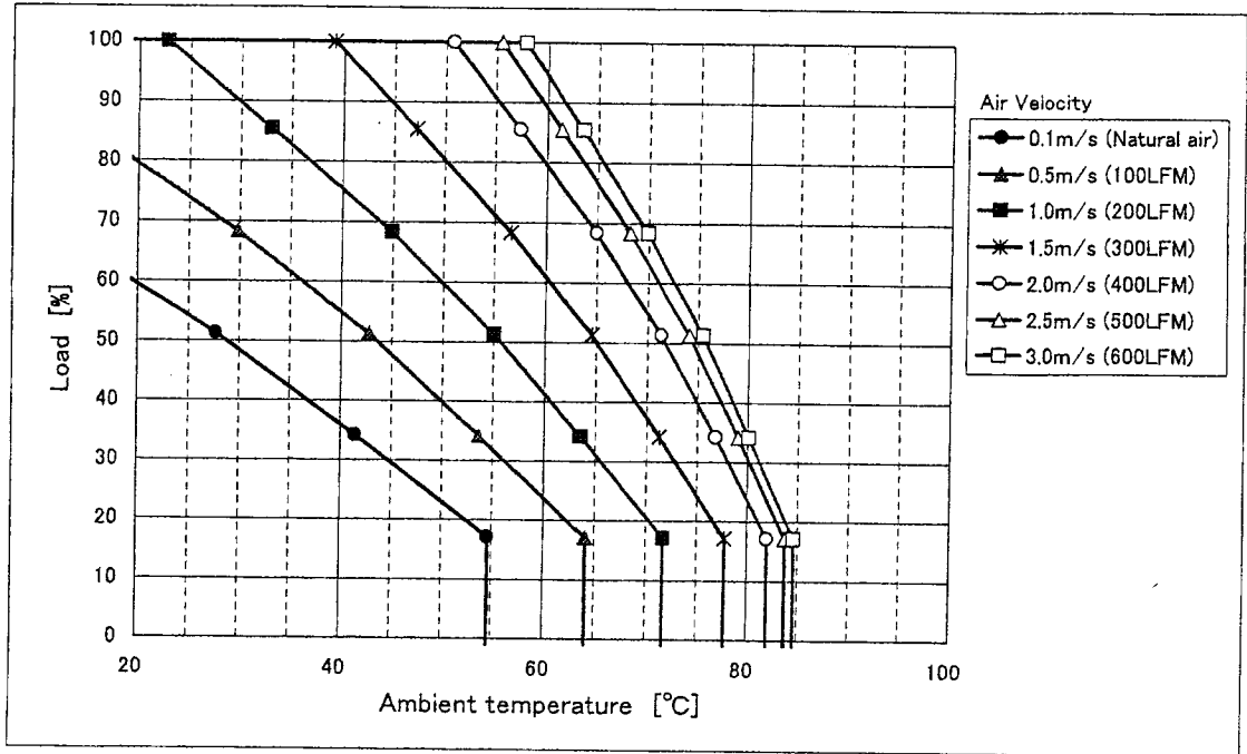
Fig. 1 CBS1004803 Derating (H=0.5inch)
