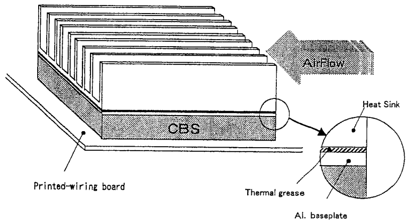
Fig.3 Test method
