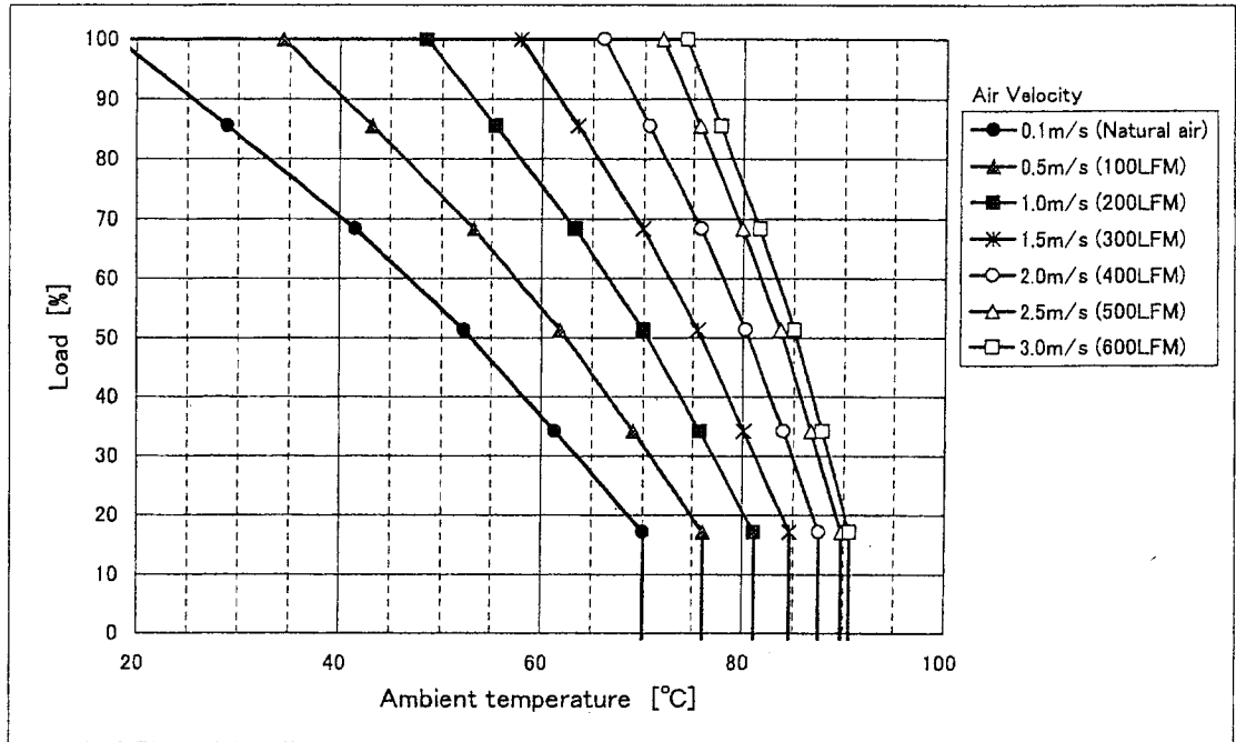
Fig. 1 CBS1004803 Derating (H=1.0inch)
