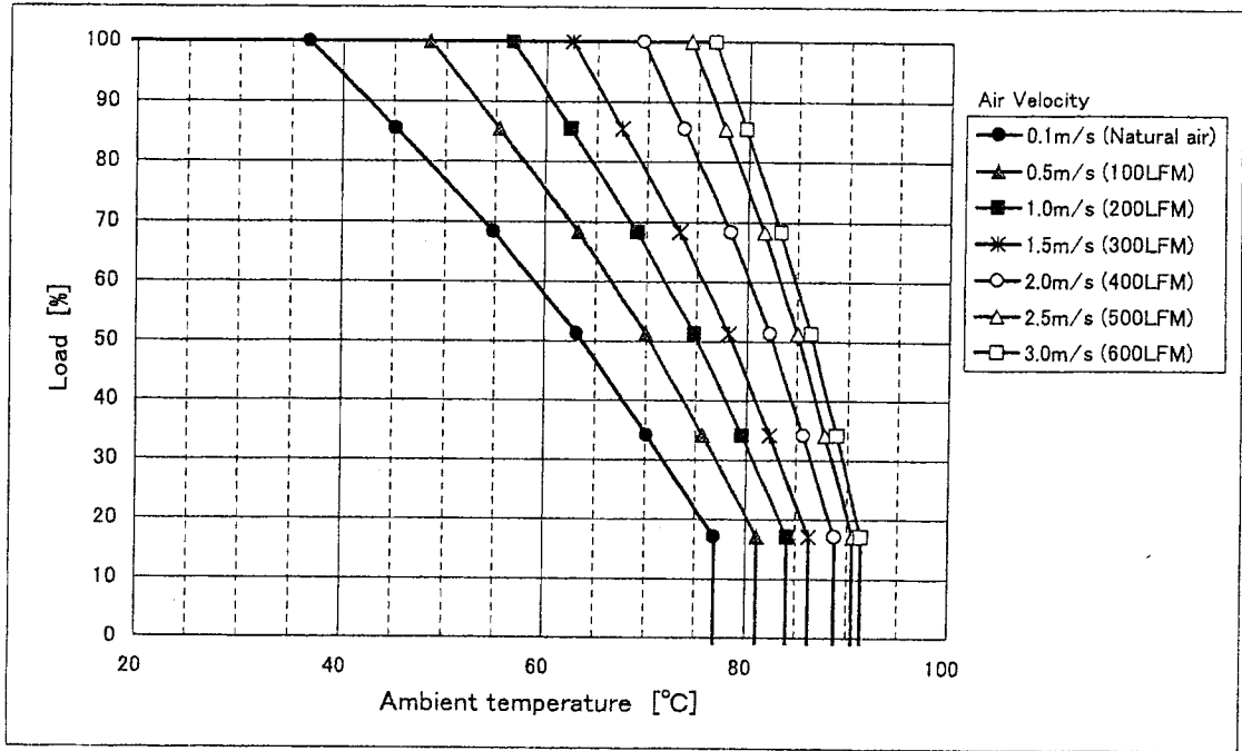
Fig. 1 CBS1004803 Derating (H=1.5inch)
