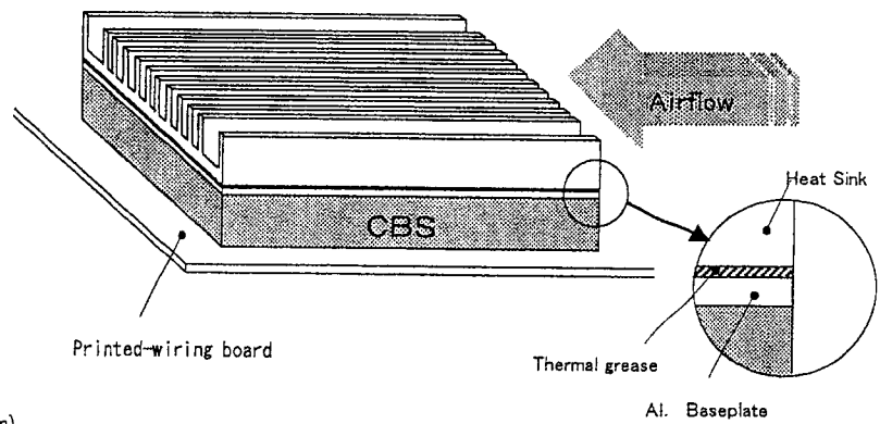
Fig.3 Test method
