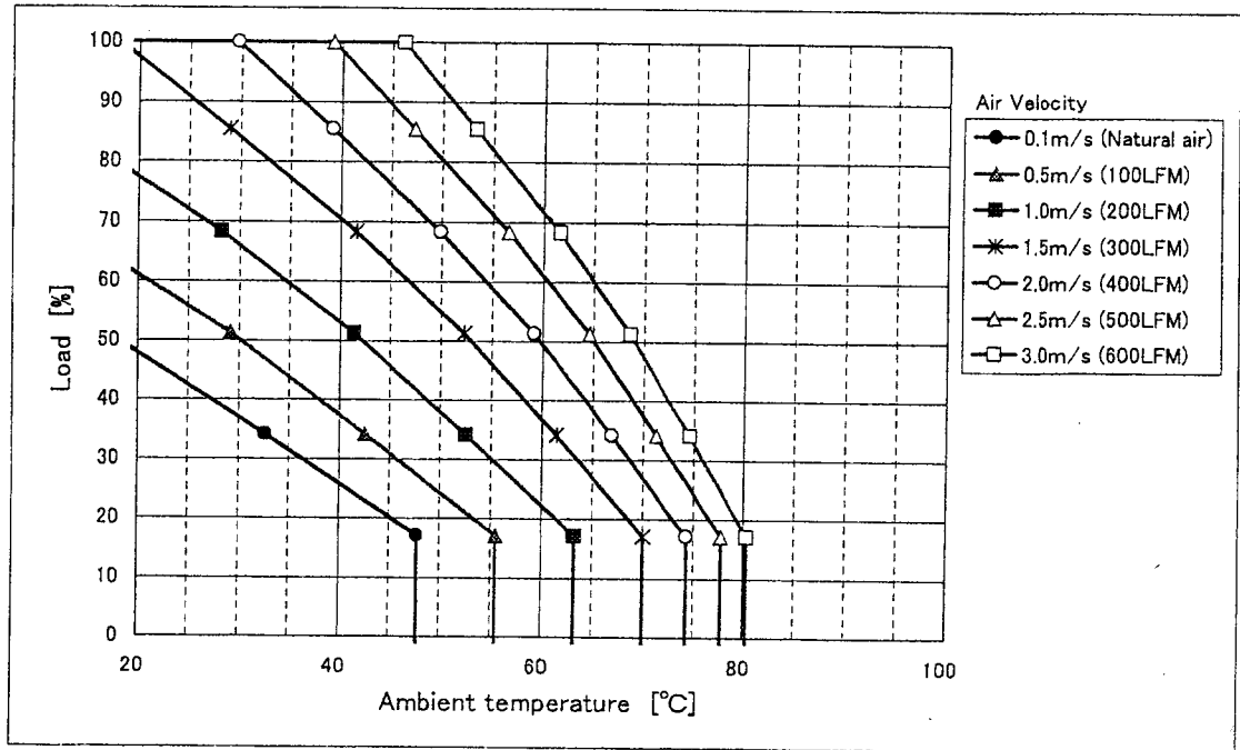
Fig. 1 CBS1004803 Derating (H=0.25inch)
