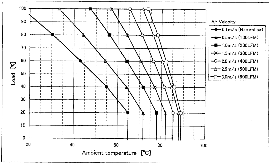
Fig. 1 CBS1004805 Derating (H=1.0inch)
