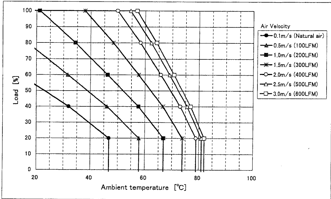
Fig. 1 CBS1004805 Derating (H=0.5inch)
