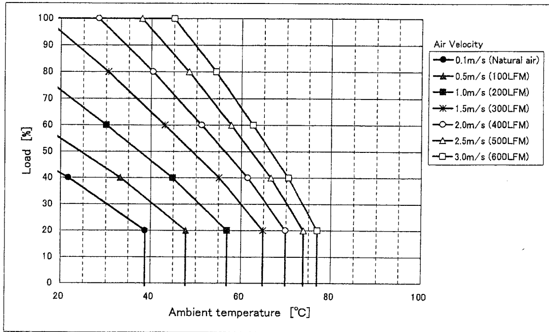
Fig. 1 CBS1004805 Derating (H=0.25inch)
