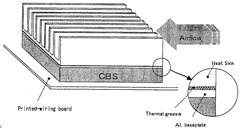
Fig.3 Test method
