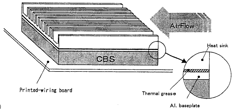
Fig.3 Test method
