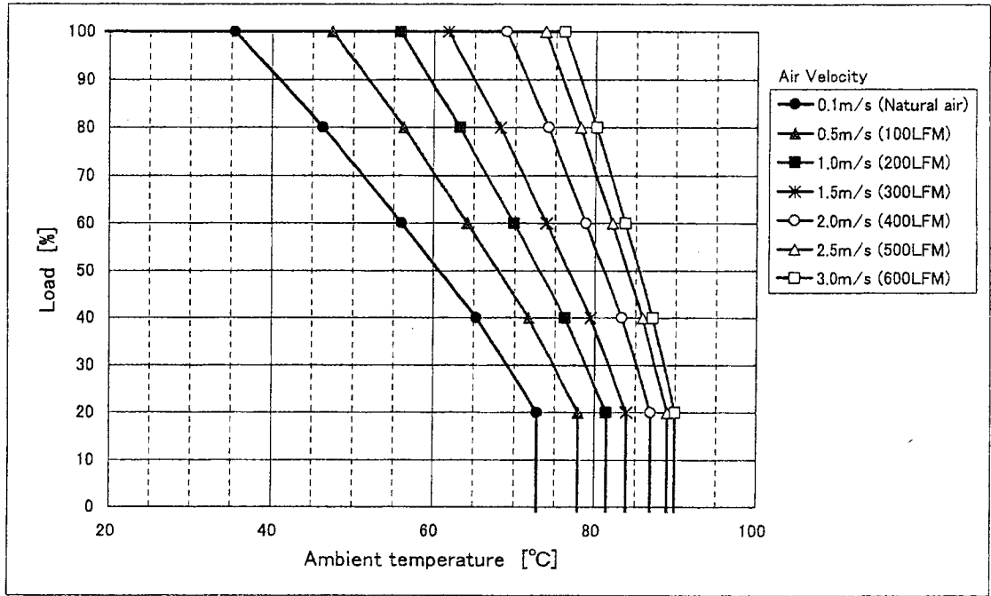
Fig. 1 CBS1004805 Derating (H=1.5inch)
