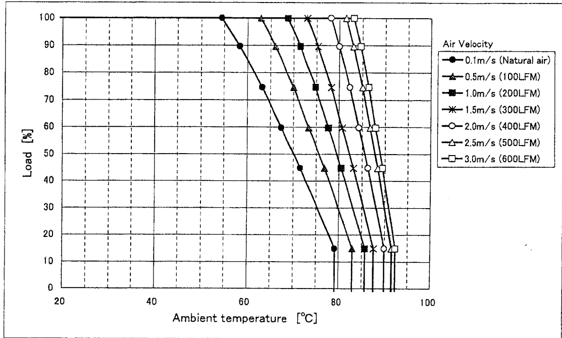
Fig. 1 CBS1004815 Derating (H=1.5 inch)
