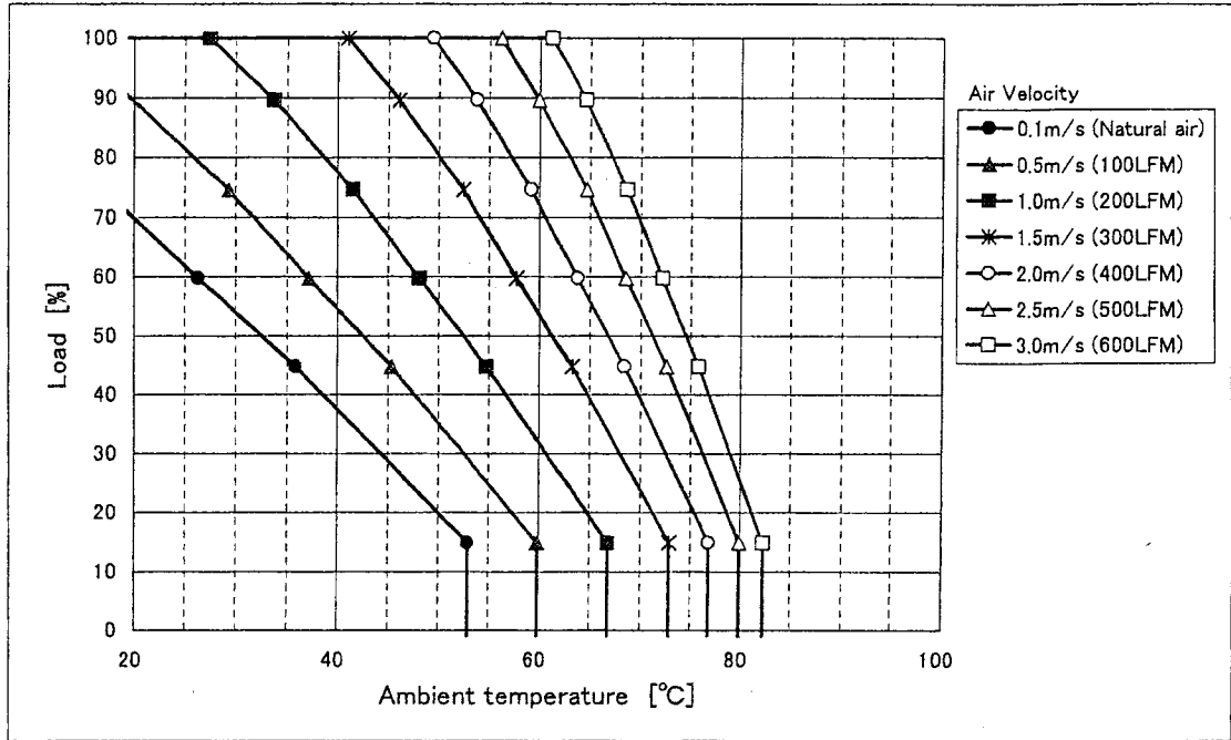
Fig. 1 CBS1004815 Derating (H=0.25inch)
