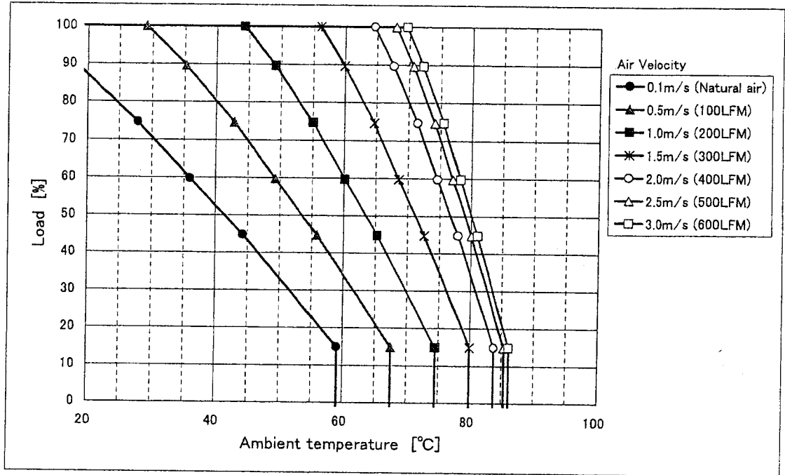
Fig. 1 CBS1004815 Derating (H=0.5inch)
