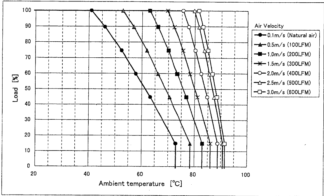
Fig. 1 CBS1004815 Derating (H=1.0inch)
