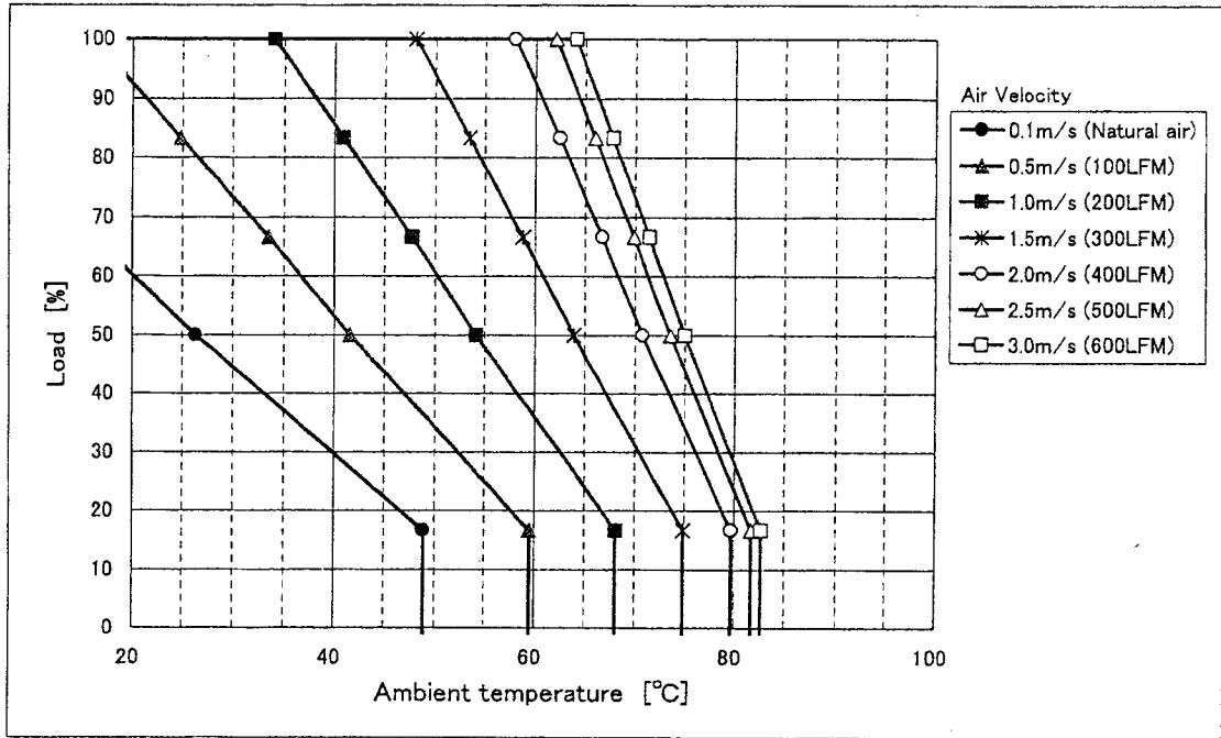
Fig. 1 CBS1004828 Derating (H=0.5inch)
