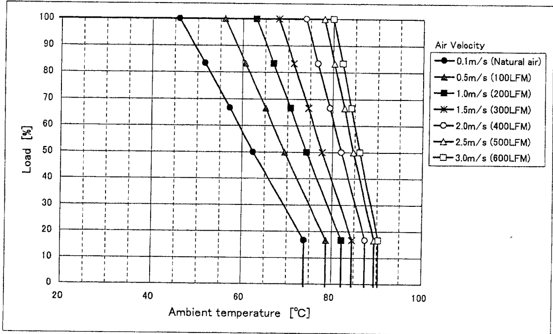
Fig. 1 CBS1004828 Derating (H=1.5inch)
