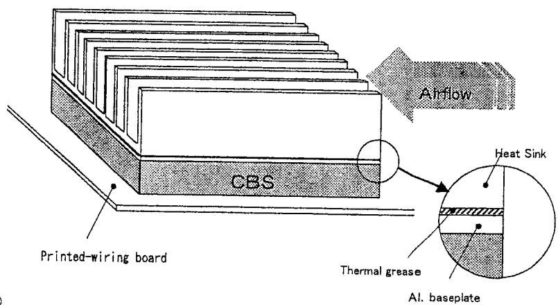
Fig.3 Test method
