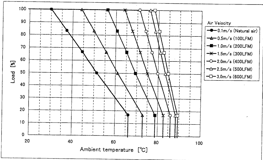
Fig.1 CBS1004828 Derating (H=1.0inch)
