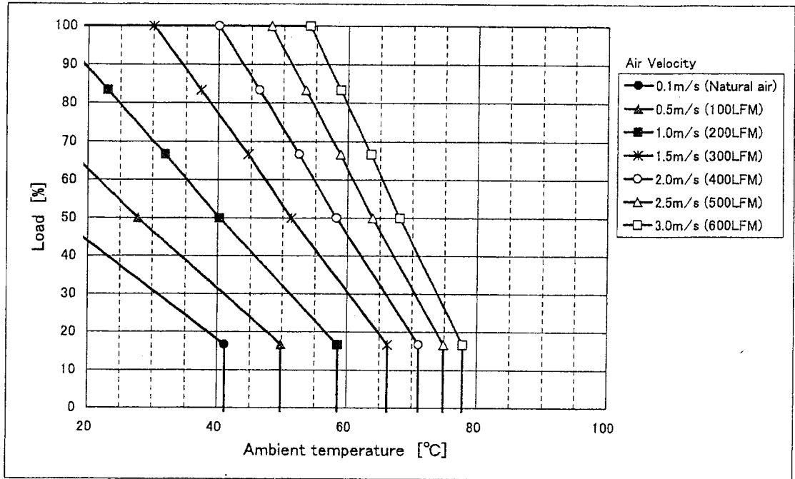
Fig. 1 CBS1004828 Derating (H=0.25inch)
