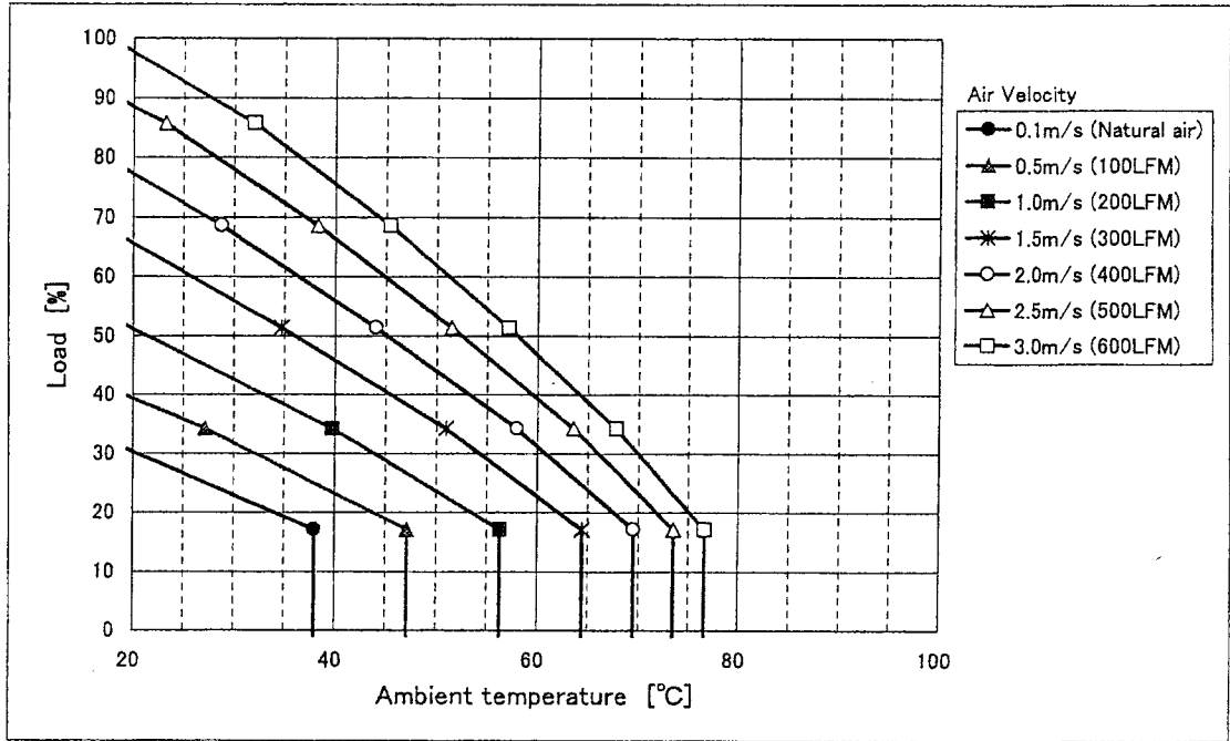
Fig. 1 CBS2004803 Derating (H=0.25inch)
