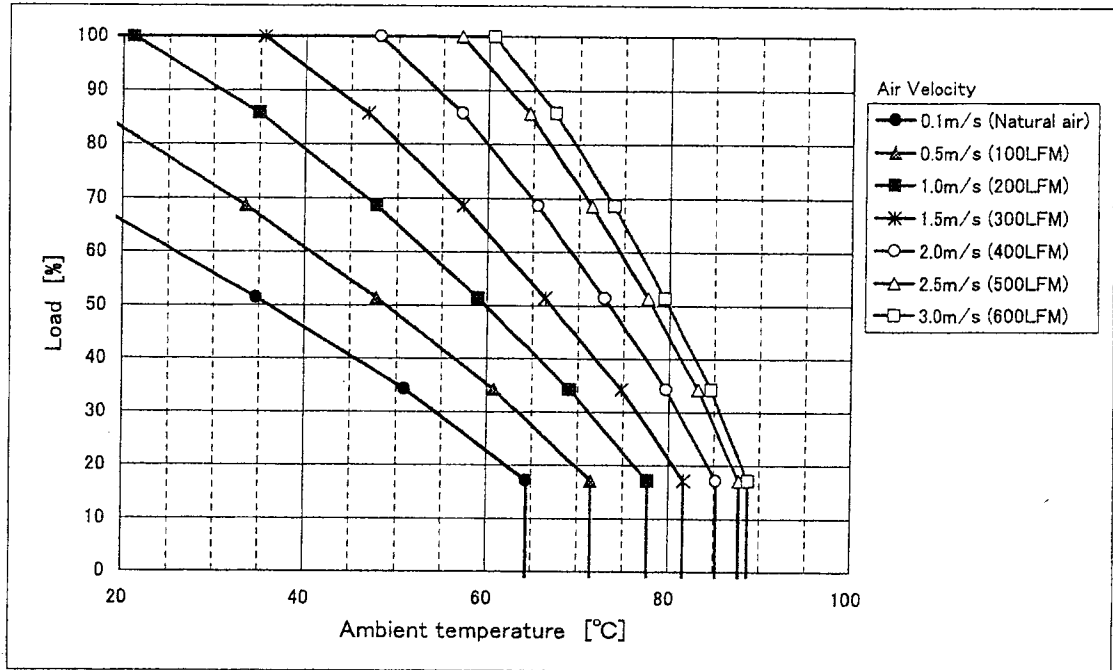
Fig. 1 CBS2004803 Derating (H=1.0inch)
