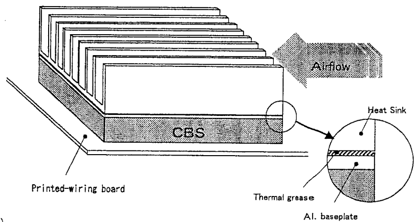
Fig.3 Test method
