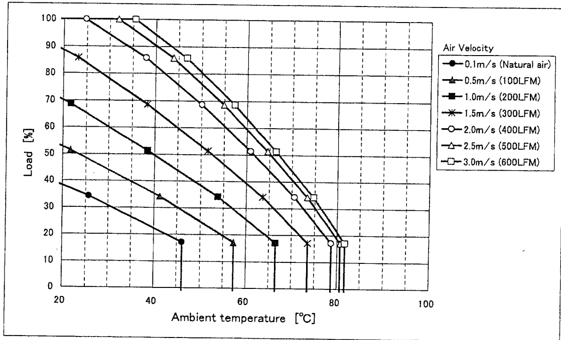
Fig. 1 CBS2004803 Derating (H=0.5inch)
