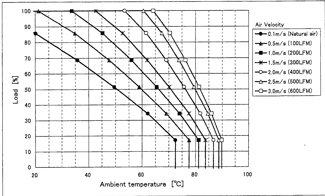
Fig. 1 CBS2004803 Derating (H=1.5inch)
