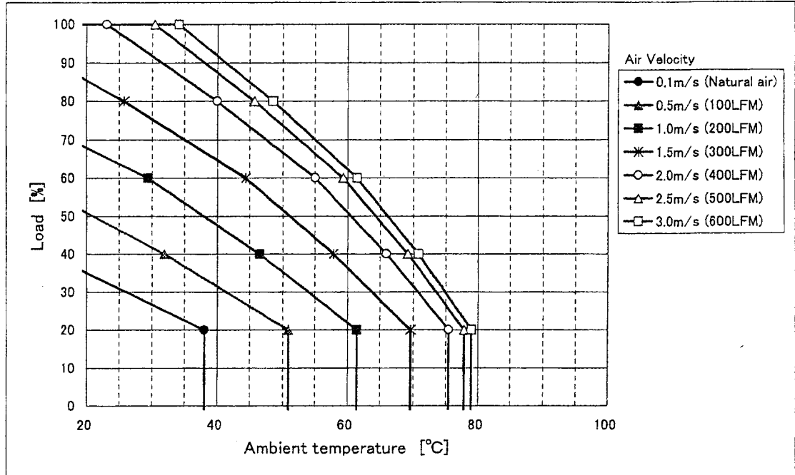
Fig. 1 CBS2004805 Derating (H=0.5inch)
