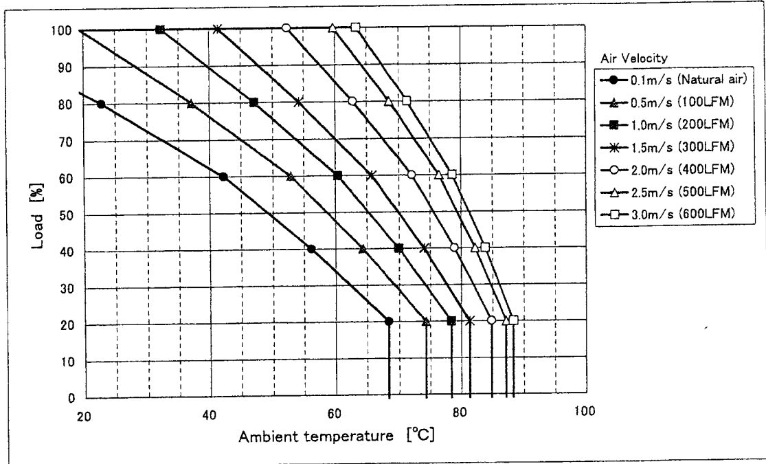
Fig. 1 CBS2004805 Derating (H=1.5inch)
