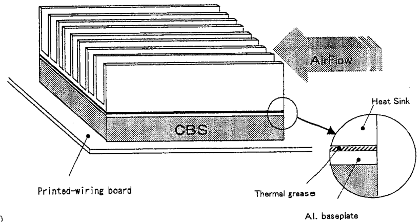
Fig.3 Test method
