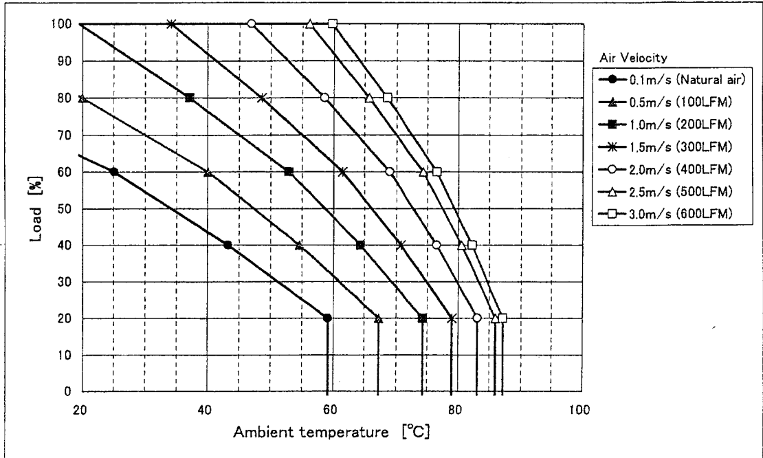
Fig. 1 CBS2004805 Derating (H=1.0 inch)
