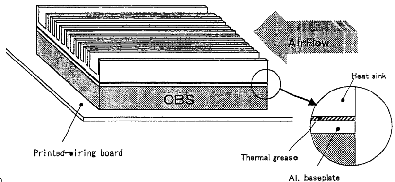
Fig.3 Test method
