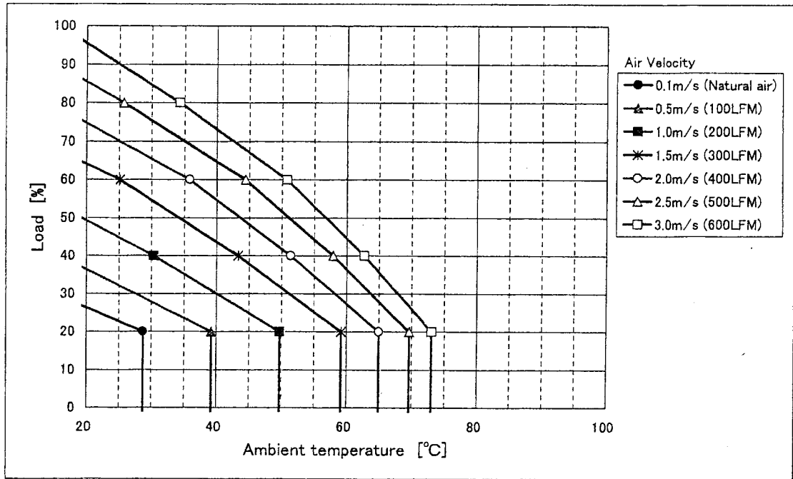
Fig. 1 CBS2004805 Derating (H=0.25inch)
