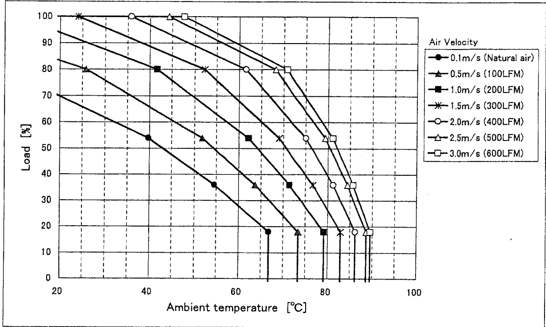
Fig. 1 CBS2004812 Derating (H=1.0inch)
