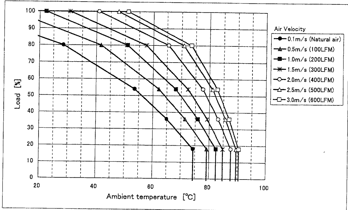
Fig. 1 CBS2004812 Derating (H=1.5inch)
