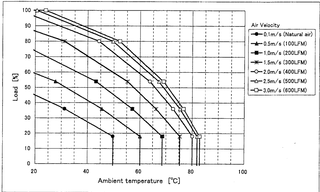
Fig. 1 CBS2004812 Derating (H=0.5inch)
