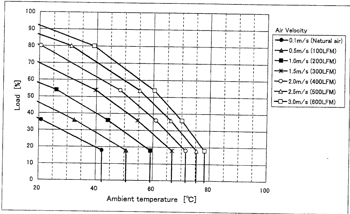
Fig. 1 CBS2004812 Derating (H=0.25inch)
