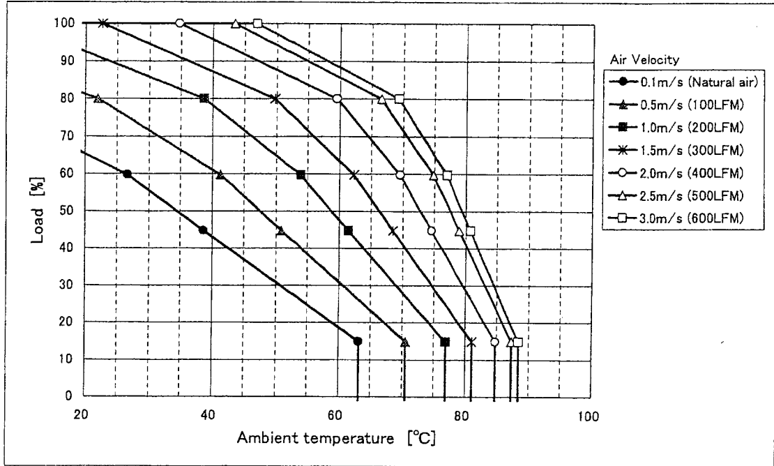
Fig. 1 CBS2004815 Derating (H=1.0inch)
