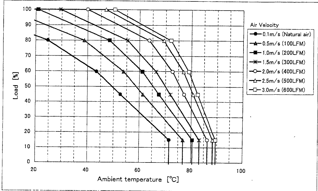
Fig. 1 CBS2004815 Derating (H=1.5inch)
