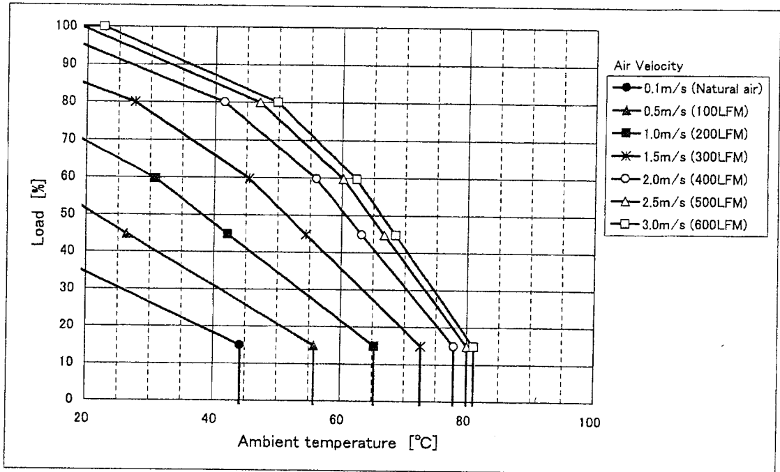
Fig. 1 CBS2004815 Derating (H=0.5 inch)
