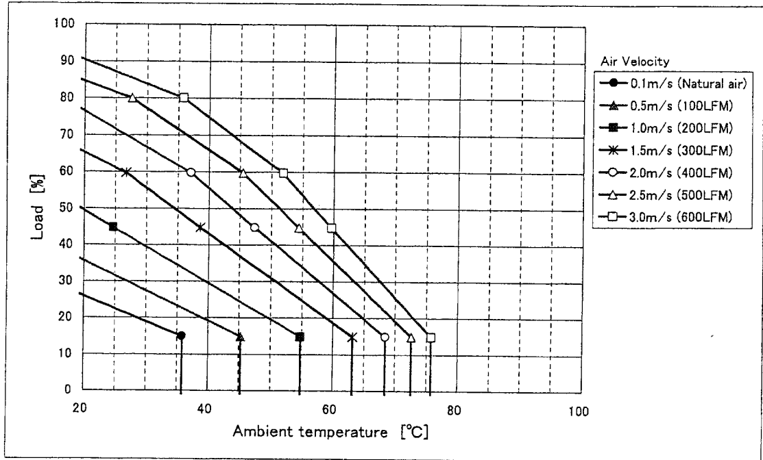
Fig. 1 CBS2004815 Derating (H=0.25inch)
