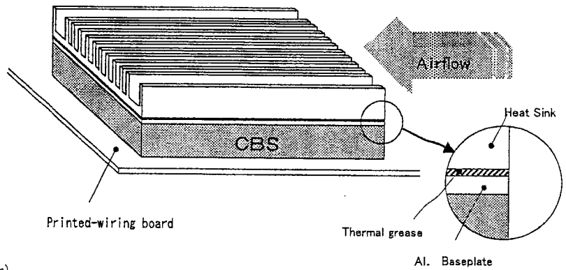
Fig.3 Test method
