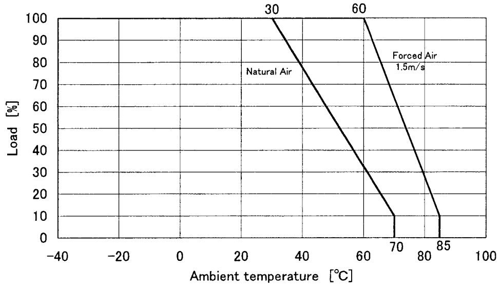
fig. 1 Derating with No Heat Sink
