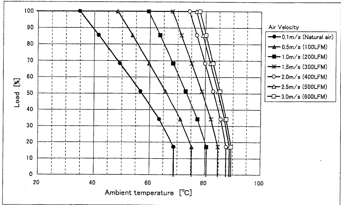
Fig. 1 CBS504803 Derating (H=0.5inch)
