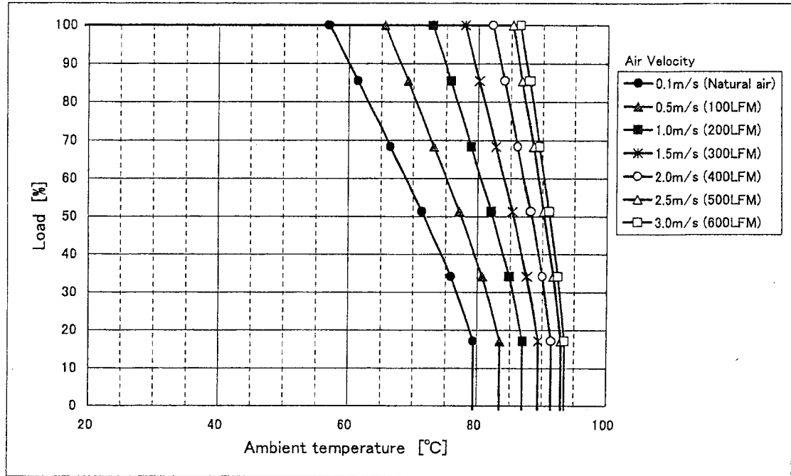
Fig. 1 CBS504803 Derating (H=1.0 inch)
