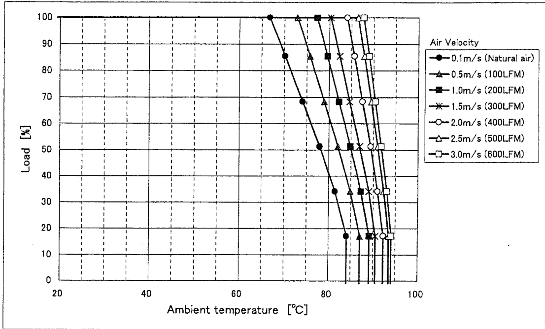
Fig. 1 CBS504803 Derating (H=1.5inch)
