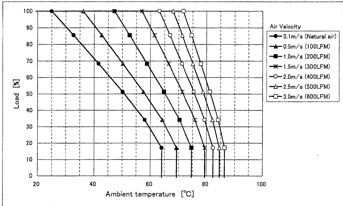
Fig. 1 CBS504803 Derating (H=0.25inch)
