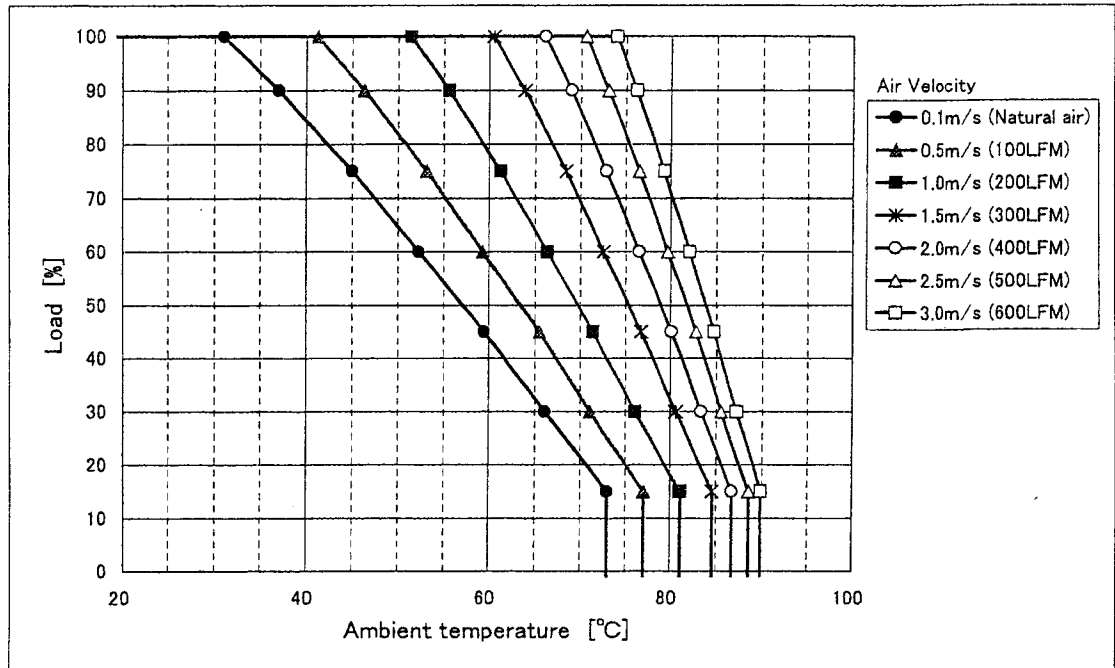
Fig. 1 CBS504805 Derating (H=0.25inch)
