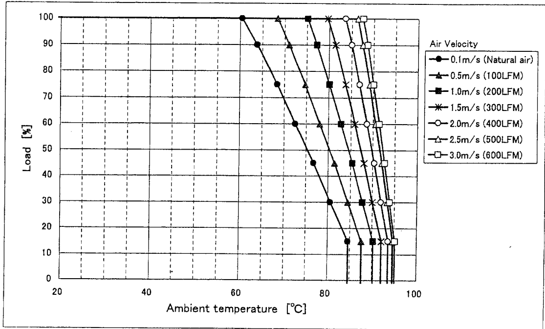
Fig. 1 CBS504805 Derating (H=1.0inch)
