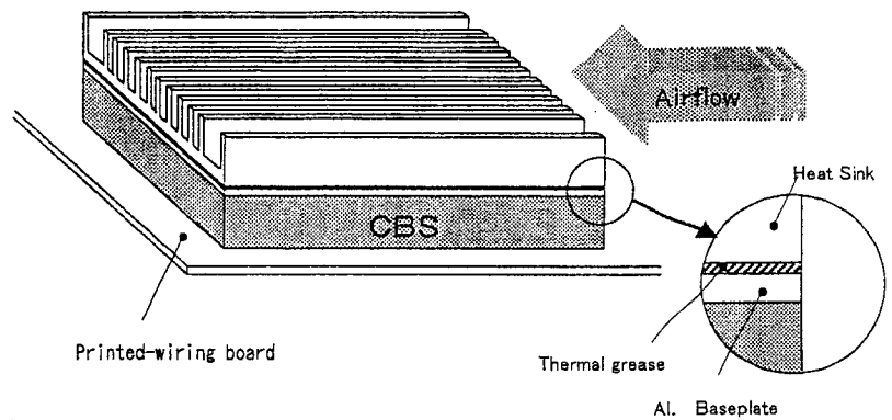
Fig.3 Test method
