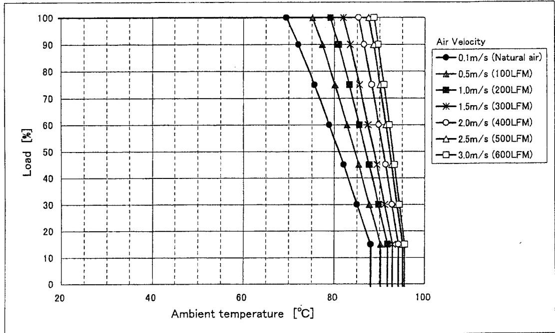
Fig. 1 CBS504805 Derating (H=1.5inch)
