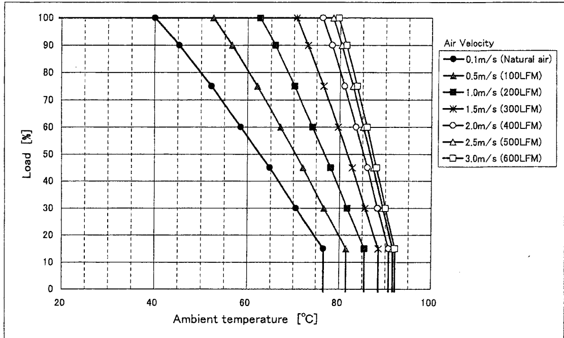
Fig. 1 CBS504805 Derating (H=0.5inch)
