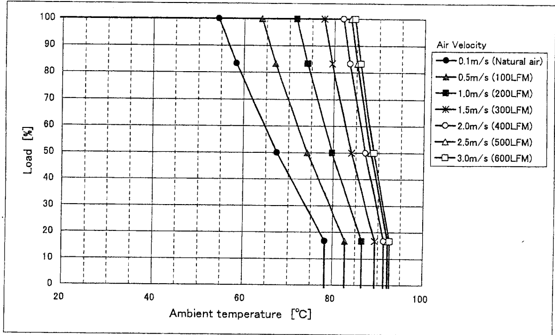
Fig. 1 CBS504828 Derating (H=0.5inch)
