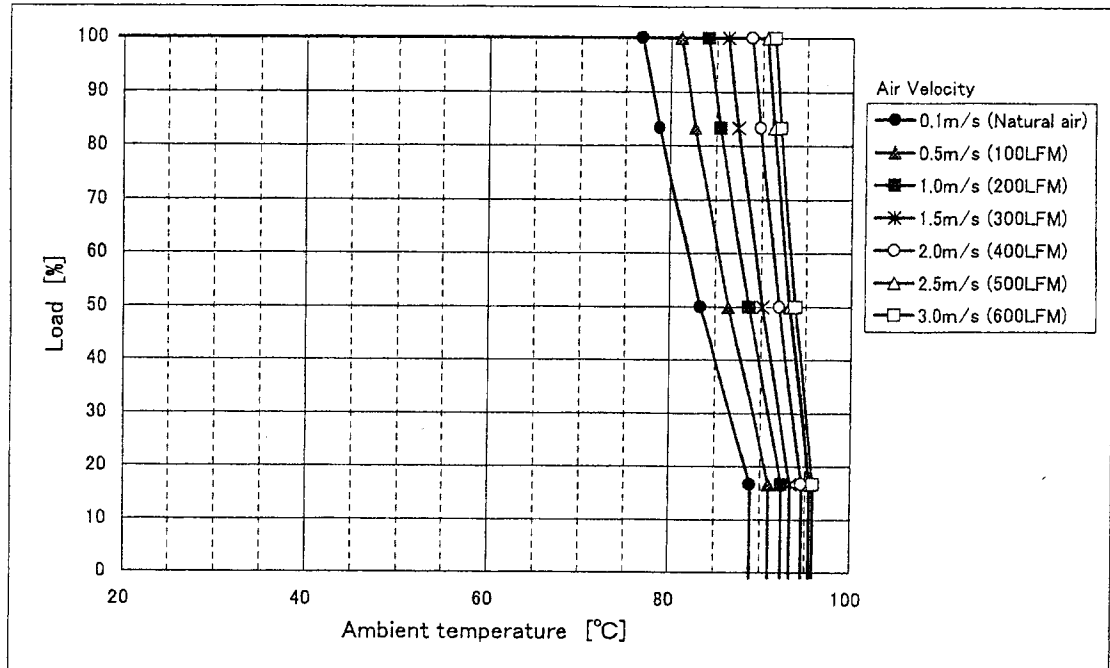
Fig.1 CBS504828 Derating (H=1.5inch)
