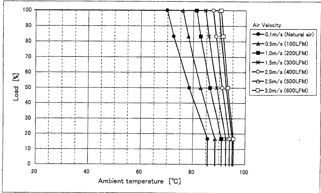
Fig. 1 CBS504828 Derating (H=1.0inch)
