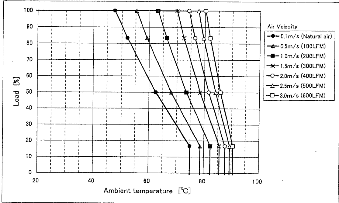
Fig. 1 CBS504828 Derating (H=0.25inch)
