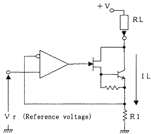
Constant current circuit
