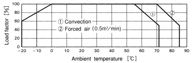
Fig.5.2 Derating curve
